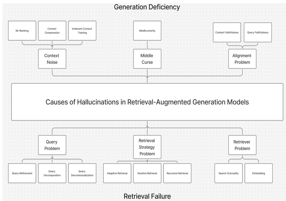
Figure 3. Causes of Hallucinations in RAG Models
