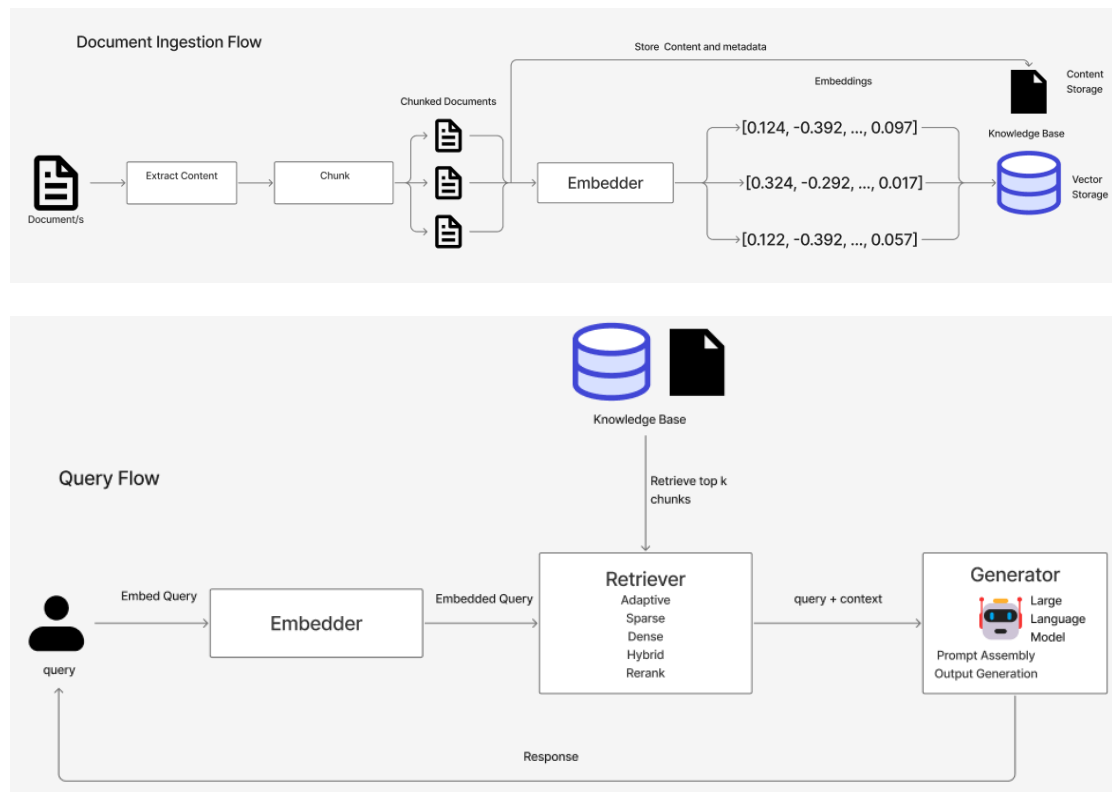
Figure 4. Overview of the RAG System
